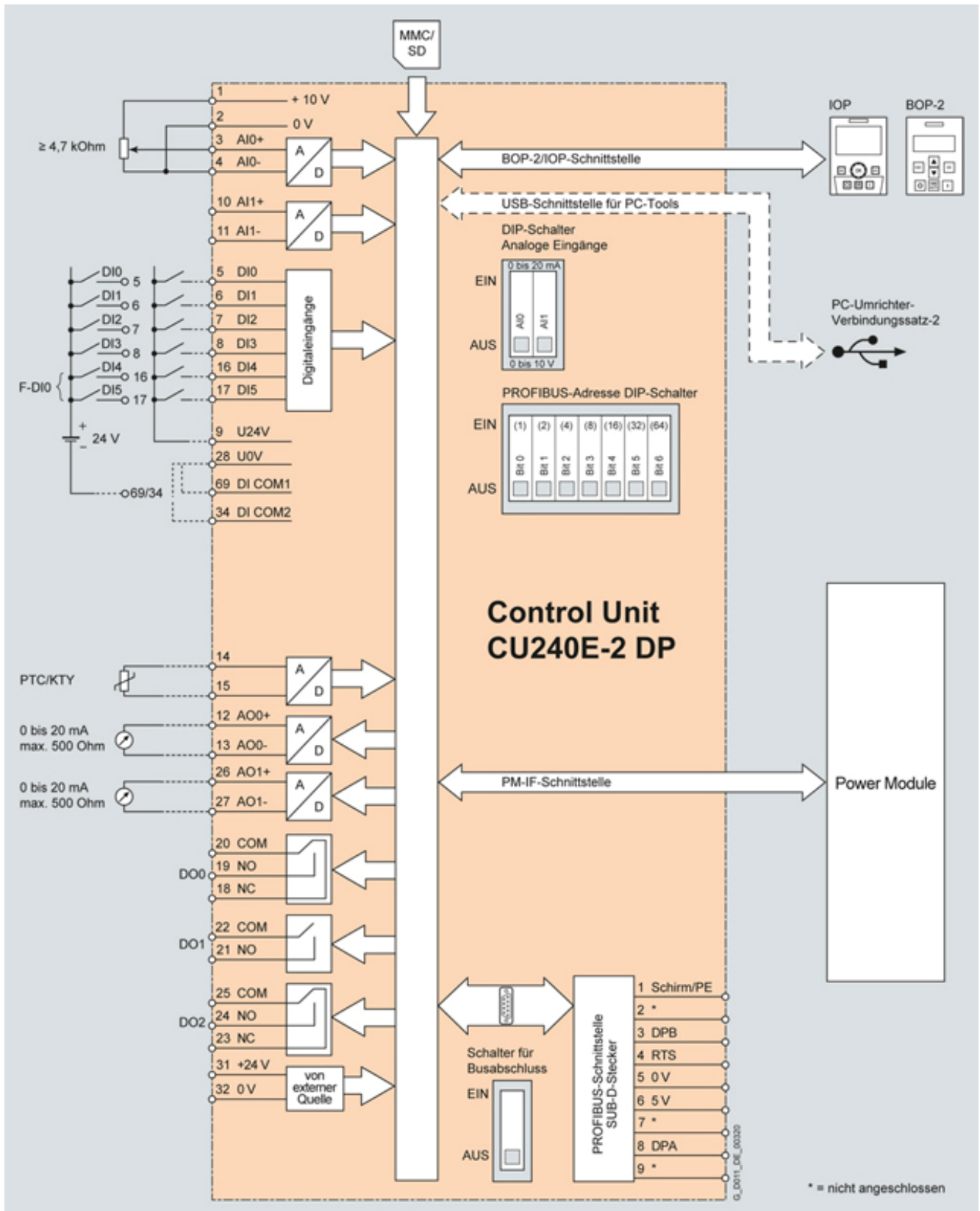
Wiring diagram for Control Unit CU240E-2 DP
