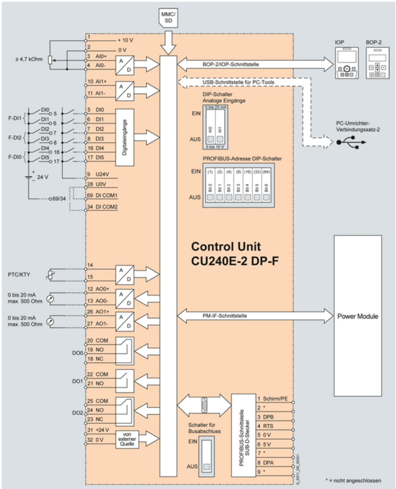
Wiring diagram for Control Unit CU240E-2 DP-F
