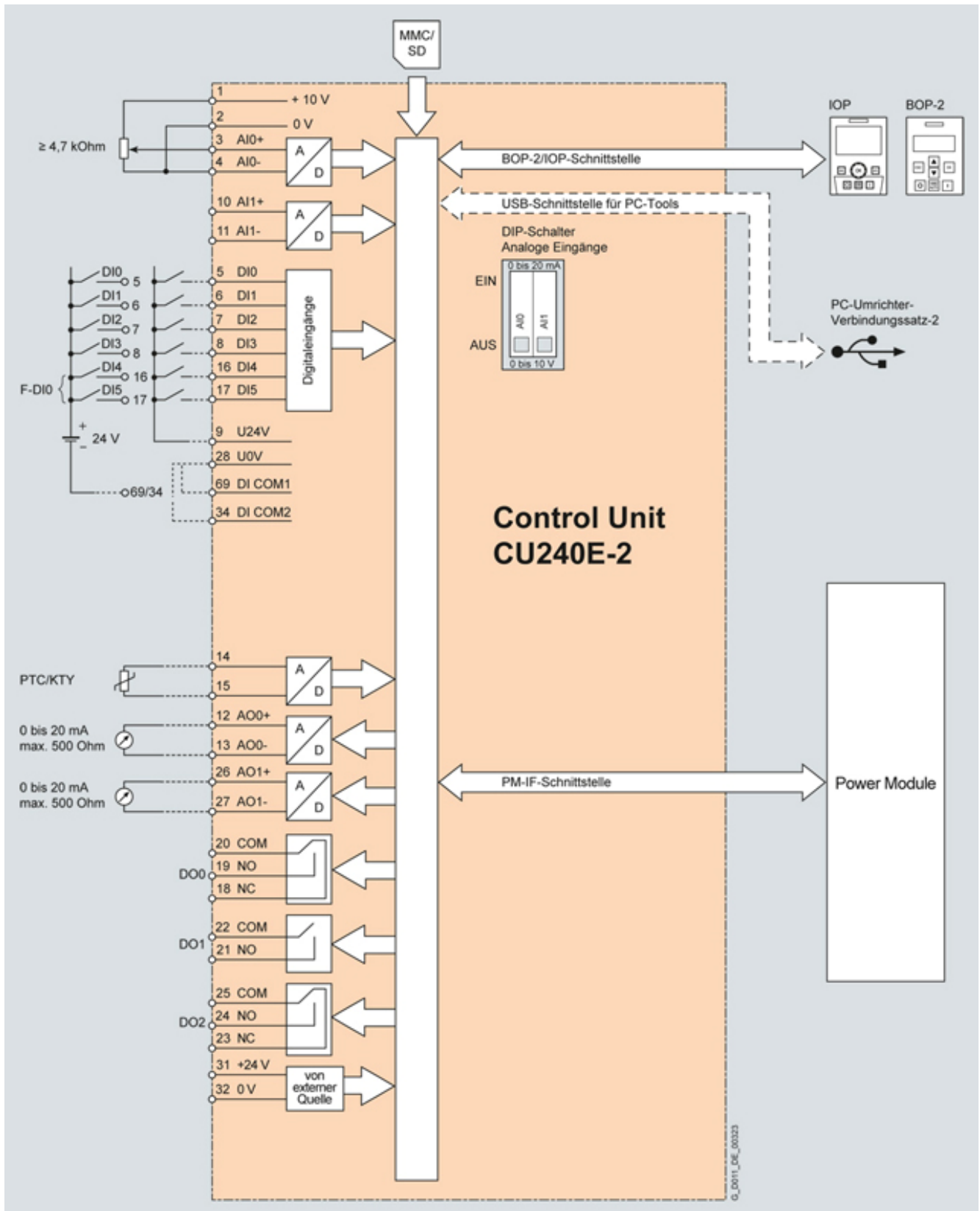
Wiring diagram for Control Unit CU240E-2
